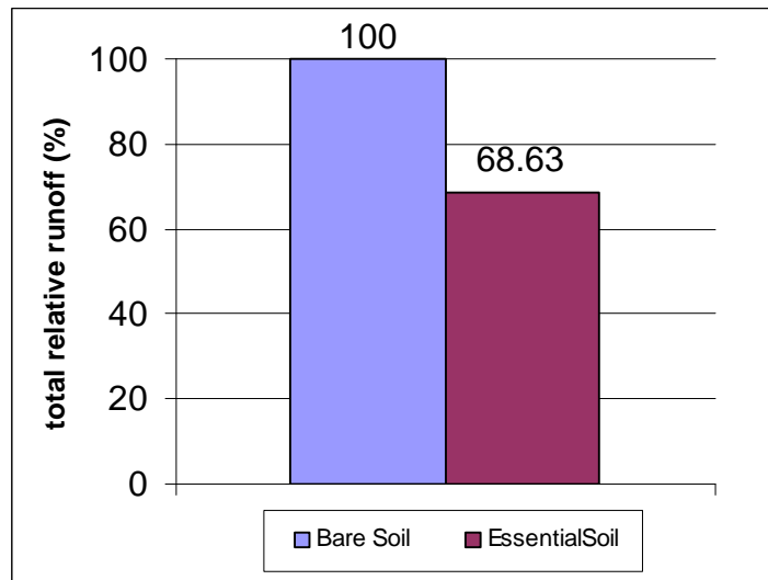
Figure 4 Comparison of Total Relative Runoff Between Bare Soil Control and EssentialSoil™
