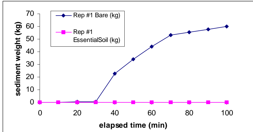
Figure 2 Comparison of Cumulative Sediment Between Bare Soil Control and EssentialSoil ®
