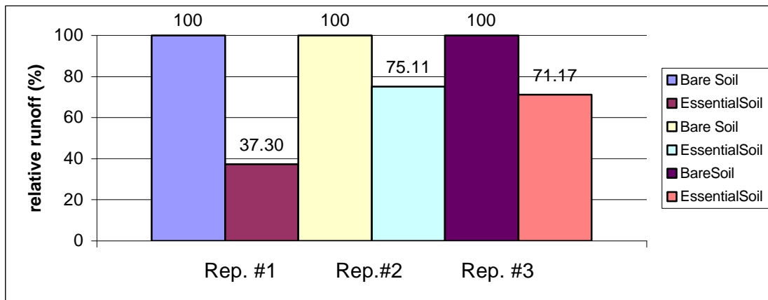
Figure 6 Runoff Volume from EssentialSoil® Treatment Expressed as Percentage of Bare Soil Control (10-year storm, three replicates)
