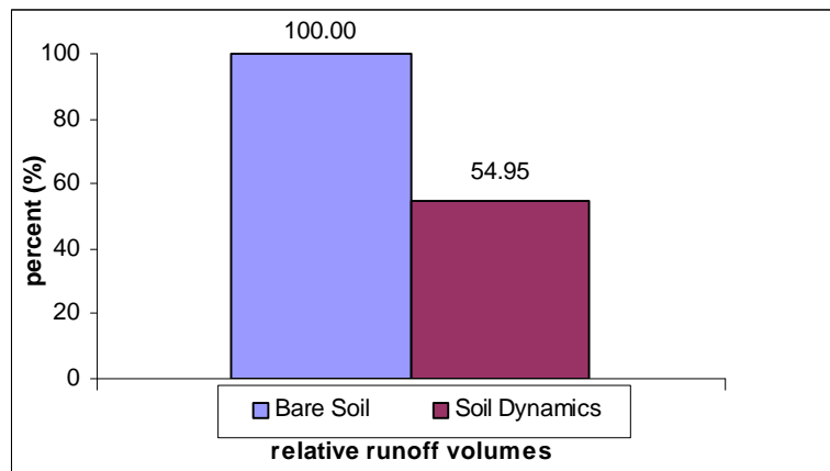
Figure 7 Comparison of Relative Runoff Between Bare Soil Control and EssentialSoil ® (50-year storm)
