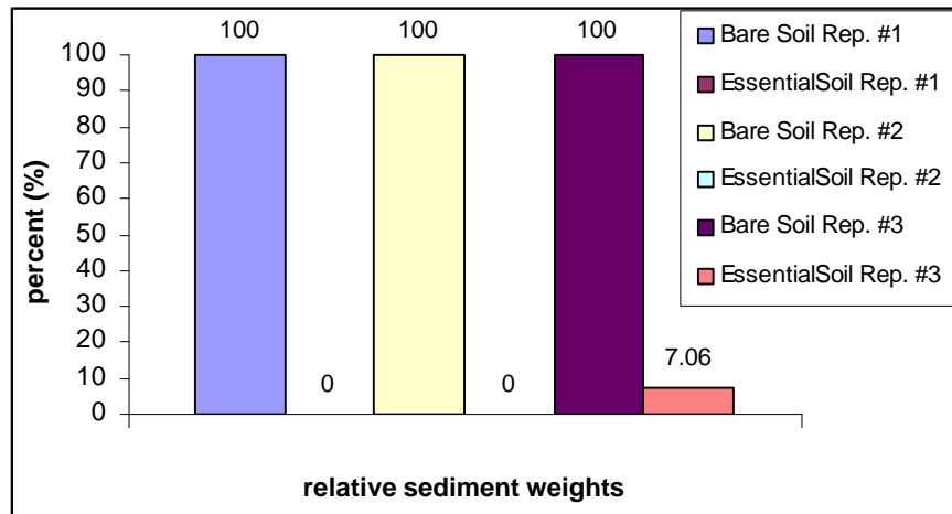
Figure 5 Dry Sediment Weight from EssentialSoil® Treatment Expressed as Percentage of Bare Soil Control (10-year storm, three replicates)
